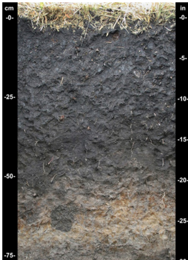
Figure 17.—Indicator A12, Thick Dark Surface. Observations deeper in the profile are needed to determine whether a soil meets the requirements of this indicator. In this soil, depth to the depleted matrix is about 55 cm.
