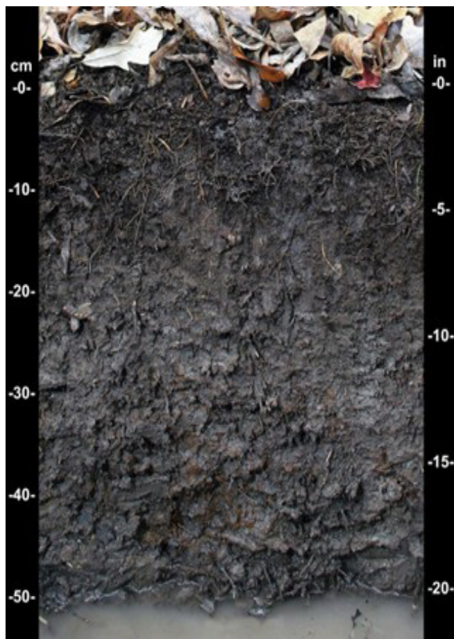
Figure 52. —The gleyed matrix in this soil starts at a depth of about 15 cm. The matrix color has value of 4 or more and is shown on one of the pages showing gleyed colors in the “Munsell Soil Color Book” (X-Rite, 2009).
