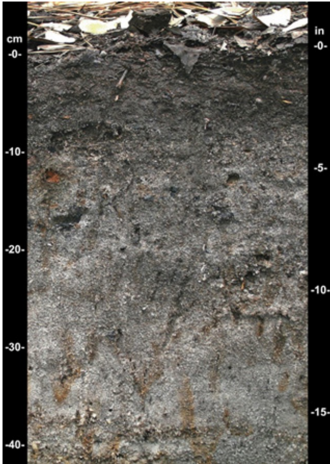
Figure 23.—Indicator S5, Sandy Redox. This soil meets the requirements of indicator S5, having a matrix chroma of 2 or less and at least 2 percent redox concentrations starting at a depth of about 10 cm.
