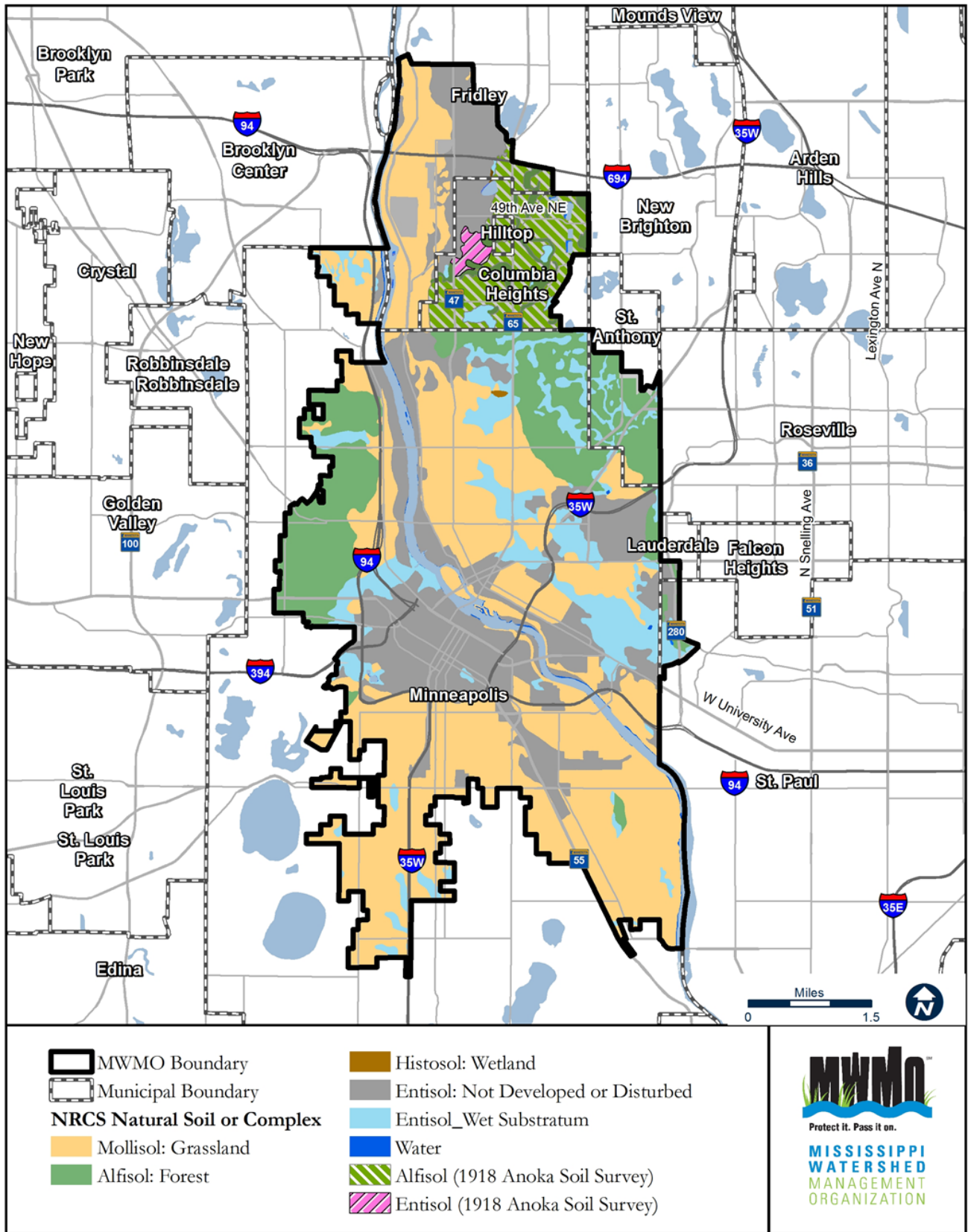
Figure 12: Soil Orders
